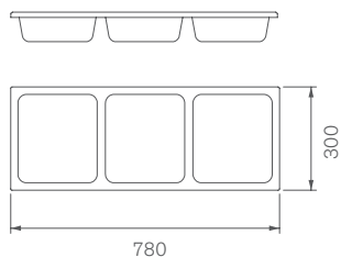
8. skålplan (vit abs plast) 78x30cm 1-pack bowl shelf (white abs plastic) 78x30cm 1-pack
