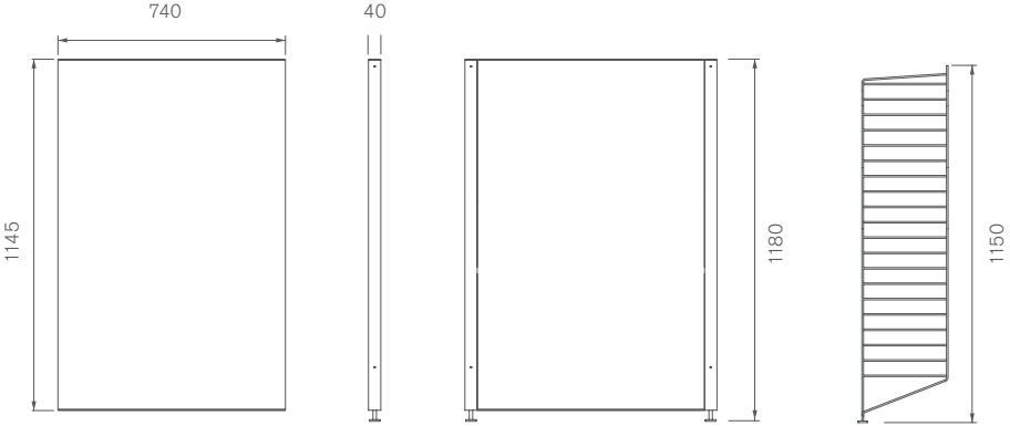
3. fristående hylla/ljudabsorberande filt // free-standing shelf/sound absorbing felt
